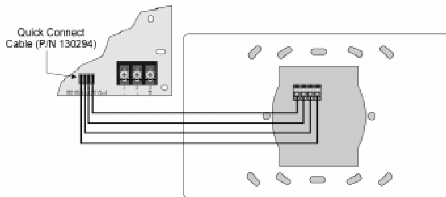
Figure 4-1 5230 Connections to the SK-2104.
