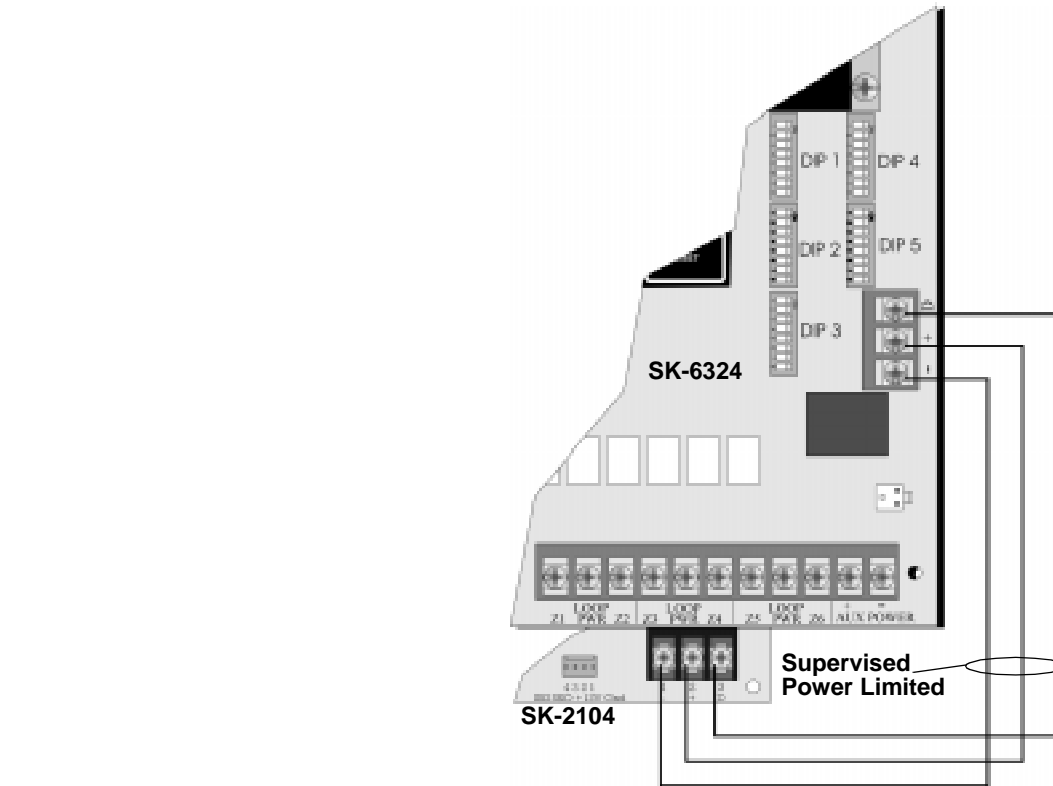
Figure 3-7 Serial Data Connections From the SK-2104 to the SK-6324
