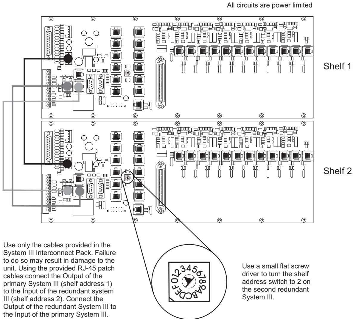
Figure 1-7, System III Redundancy Wiring Diagram
