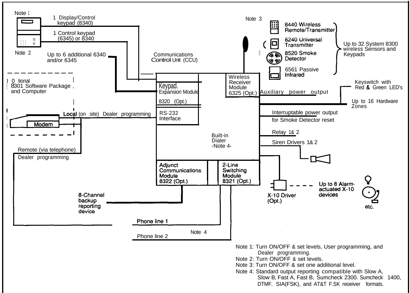
Figure I-1 System Diagram
