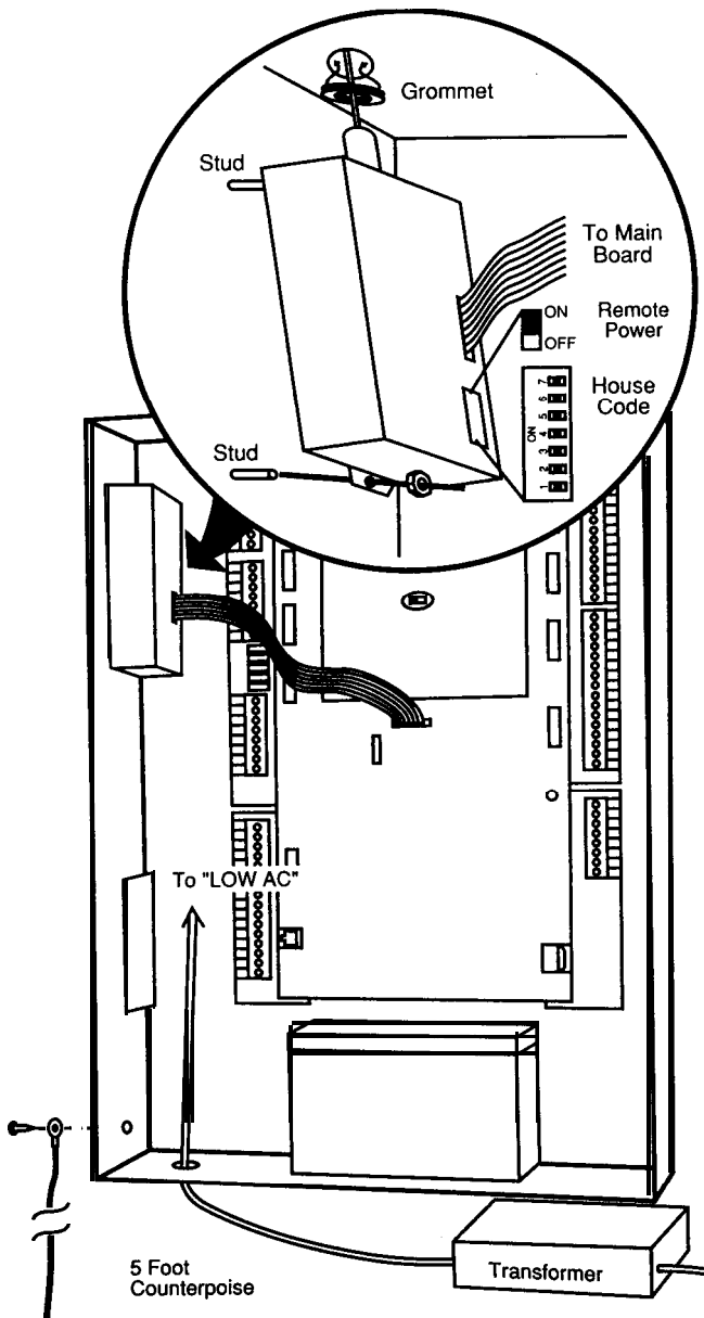
Figure A-2 Wireless Module
