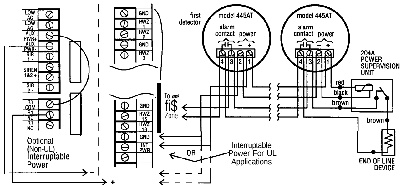
Figure 2-17 Hardwired Smoke Detectors
