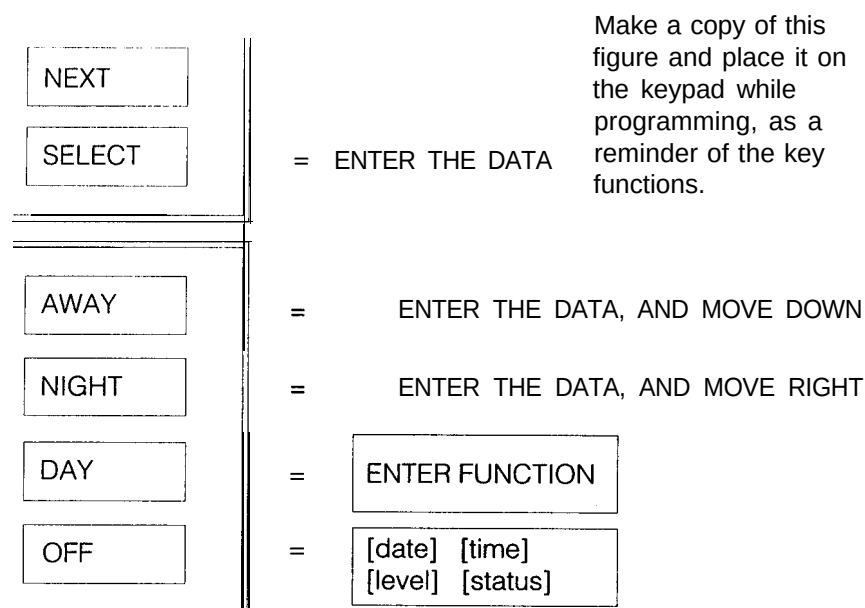
Figure 3-3 Keypad Button Functions
