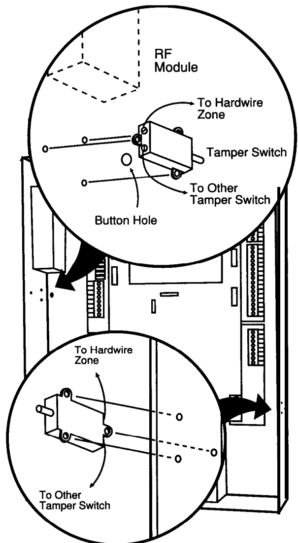
Figure 2-9 Tamper Switches
