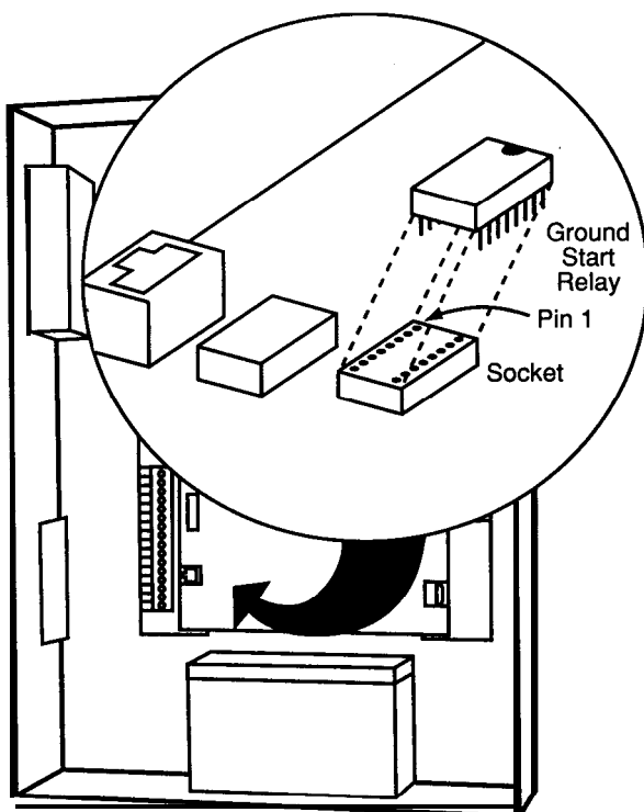
Figure 2-8 Ground Start Relay
