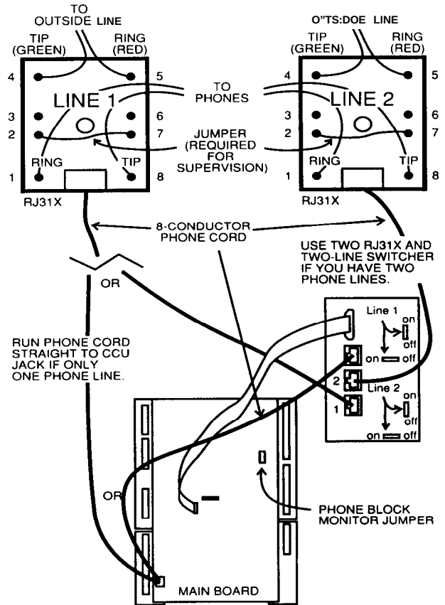
Figure 2-11 Supervision with RJ-31X
