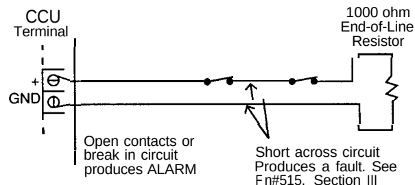
Figure 2-3 Closed Loop (Fn#515 = 0)
