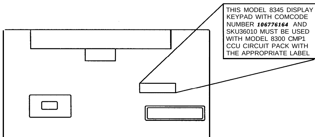
Figure 2-13b. Display Control Keypad
