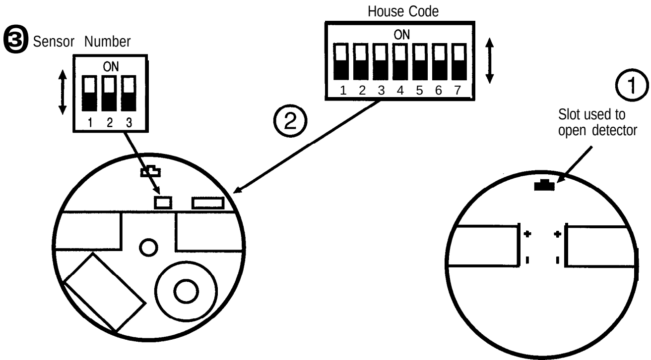
Figure A-6 Smoke Detector (Model 8520)
