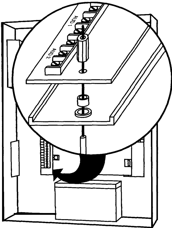
Figure 2-12 Expansion Module
