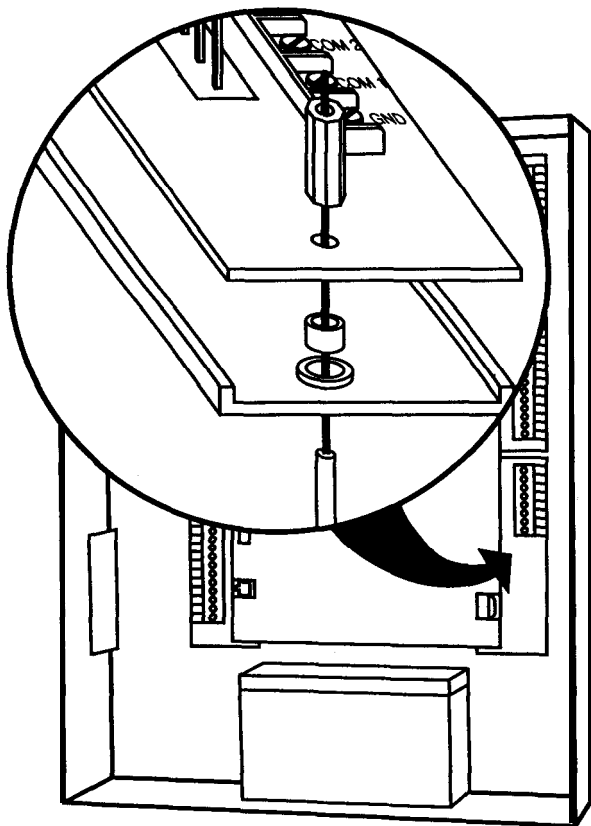
Figure 2-13 Adjunct Communicator Module
