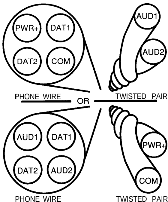
Figure 2-1 Non-UL Wiring Options
