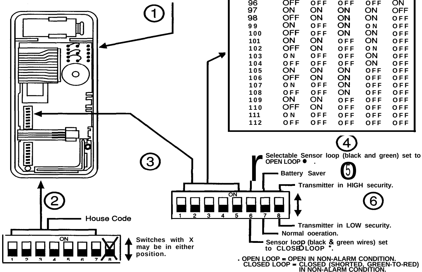
Figure A-4 Remote Transmitter
