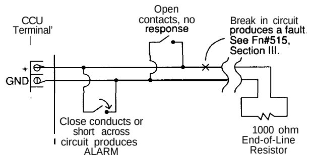
Figure 2-2 Open Loop (Fn#515 = 1)
