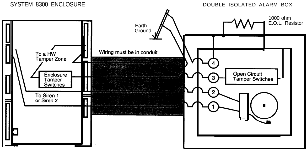
Figure 2-18 UL Bell Wiring
