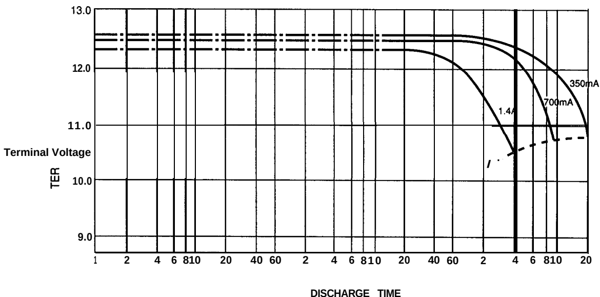
Figure 2-6 Typical Battery Life vs. Current, for 7 Amp-Hour Battery
