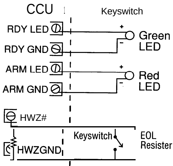
Figure 2-16 Open Loop Keyswitch
