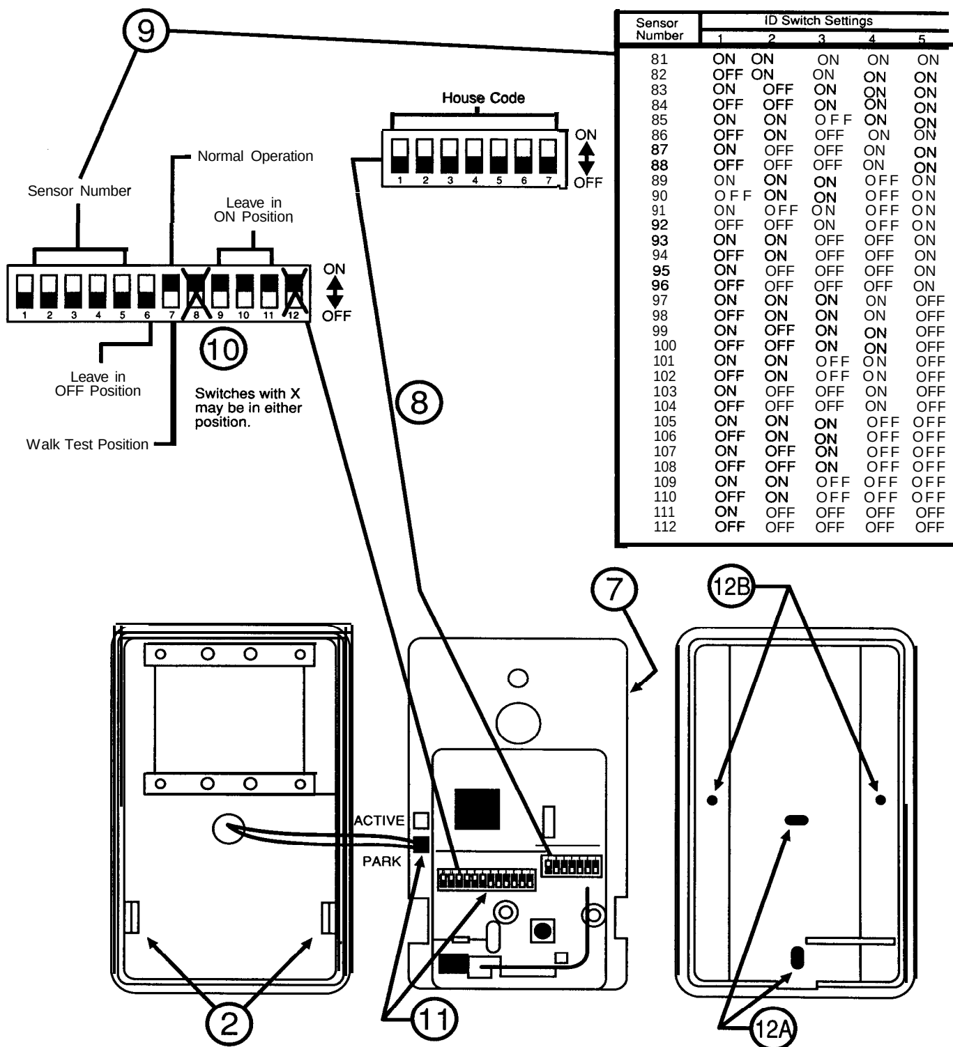
Figure A-7 Passive Infrared Detector (PIR)
