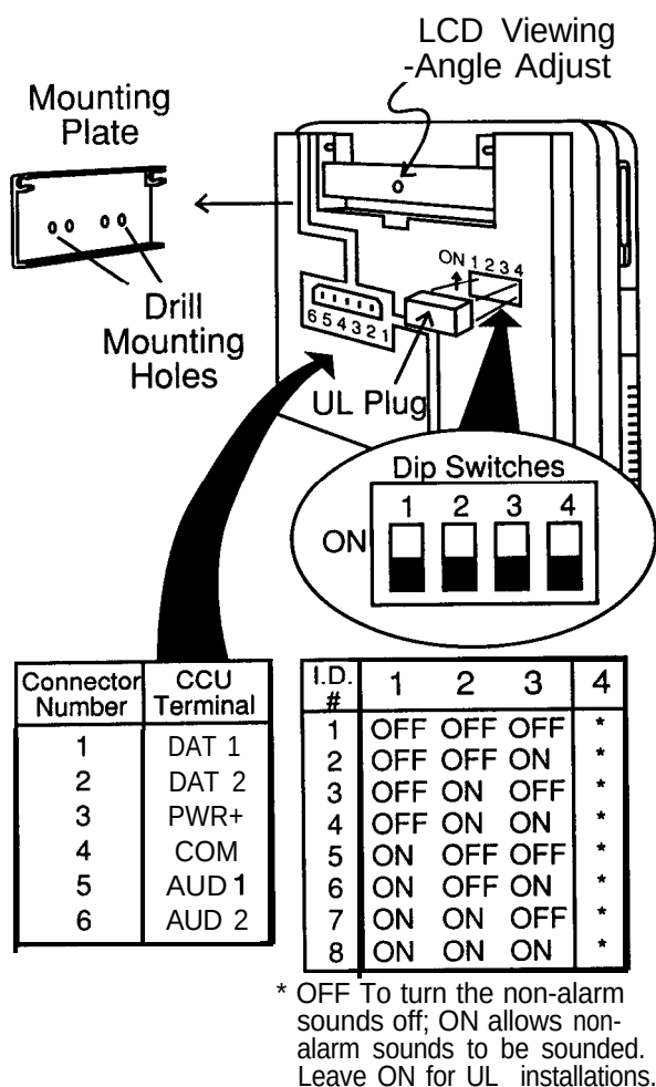
Figure 2-15 Keypad Settings and Connections
