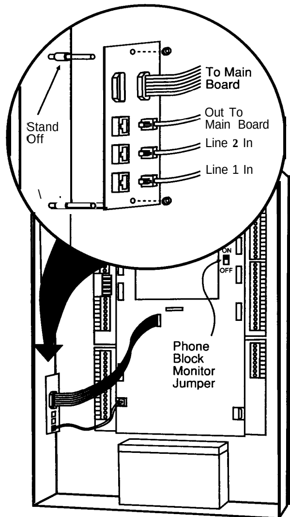
Figure 2-10 Two-Line Switcher
