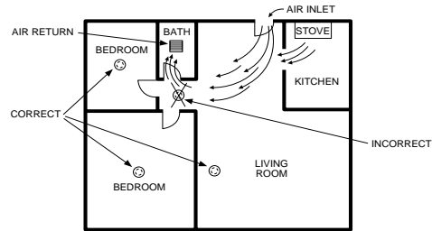
Figure 5. Recommended smoke detector locations to avoid air streams with combustion particles
