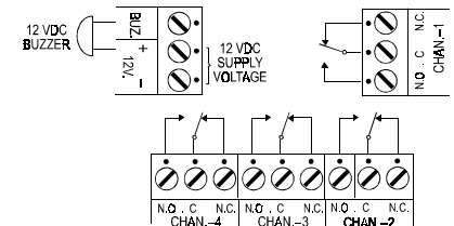
Figure 7. WR-200/4B Wiring
