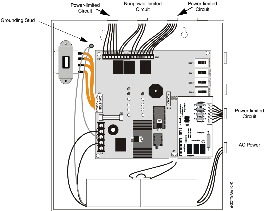
FIGURE 2-9: Typical Wiring Diagram for UL Power-limited Requirements
