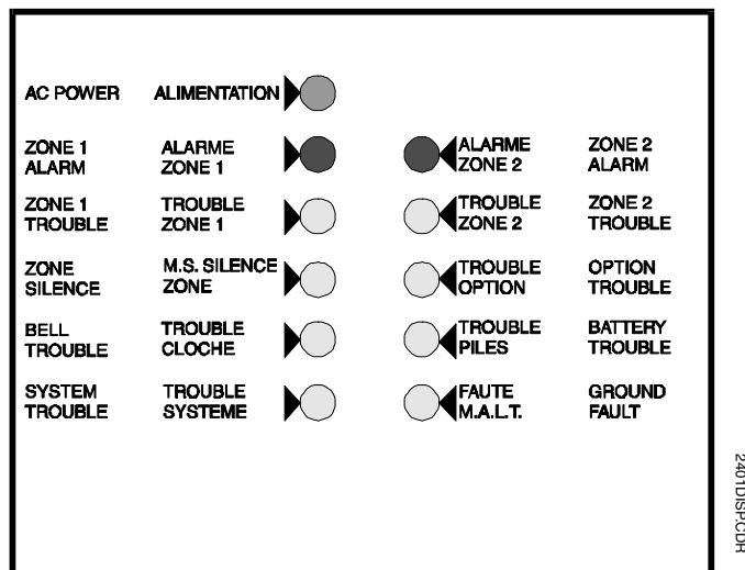
FIGURE 1-3: LED Indicators (CMP-2402B Illustrated)
