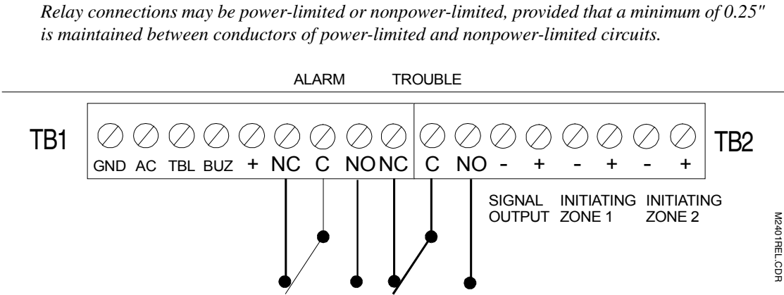
FIGURE 2-8: Relay Terminals
