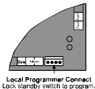
Figure 9: Programmer Jack
