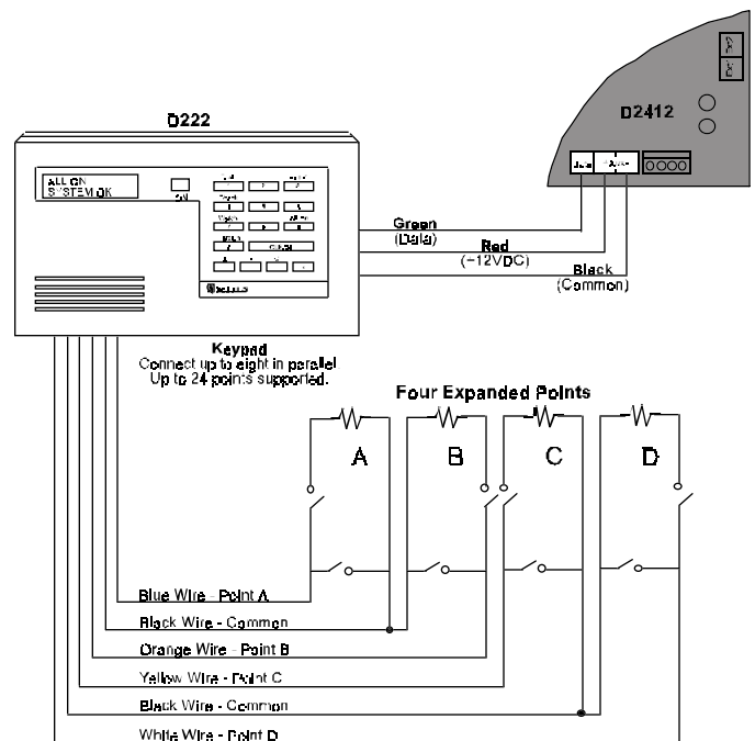
Figure 3: Keypad Wiring
