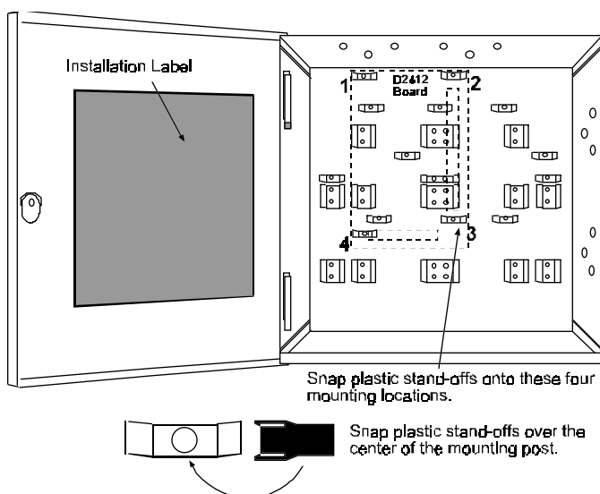
Figure 1: D2203 Enclosure
