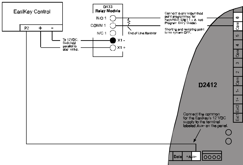
Figure 13: Keyswitch
