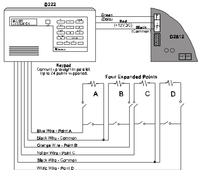
Figure 3: Keypad Wiring
