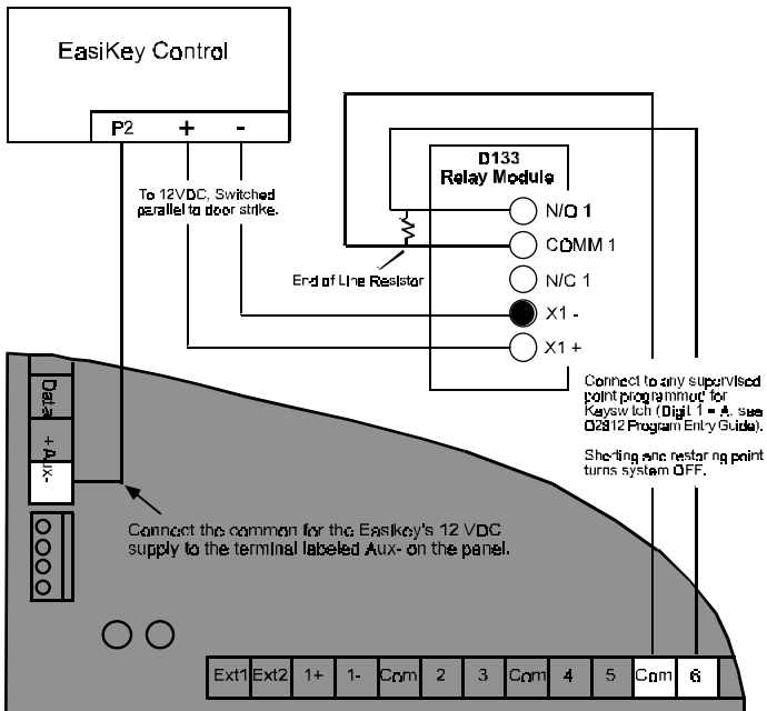
Figure 13: Keyswitch
