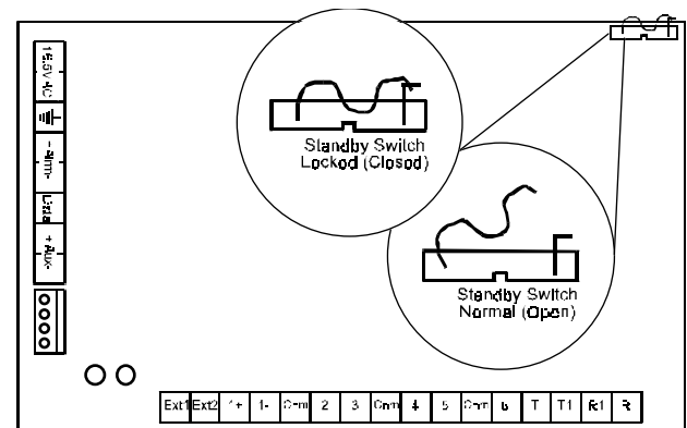
Figure 2: Standby Switch
