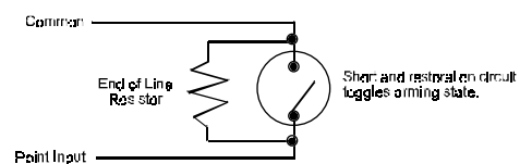
Figure 12: Keyswitch
