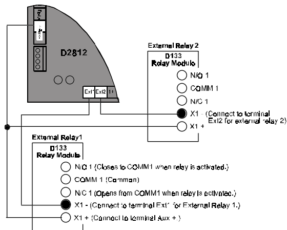
Figure 4: External Relay Wiring
