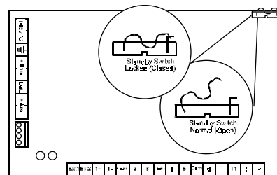
Figure 8: Standby Switch
