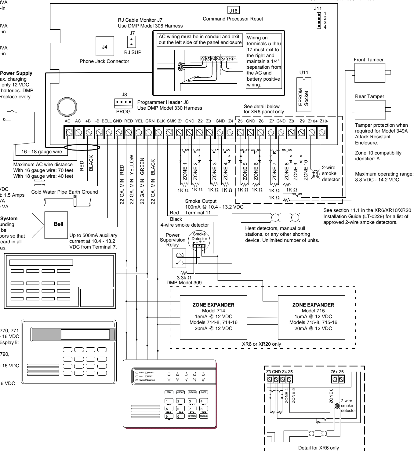
Figure 1: XR6/XR10/XR20 wiring diagram
